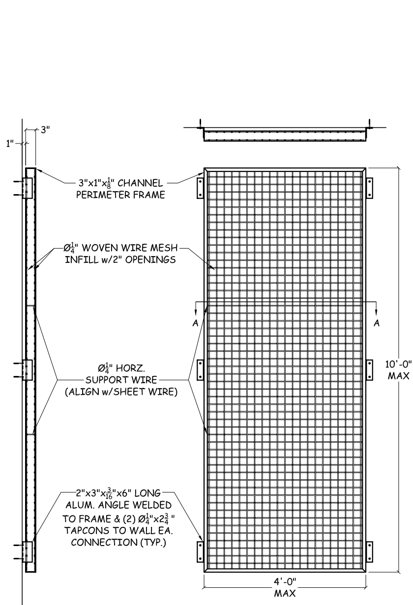
G-GS1 WALL MOUNT ALUM GREEN SCREEN
