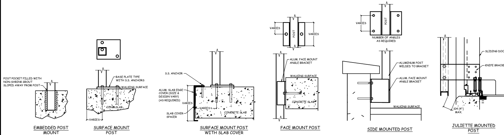
MOUNTING OPTIONS
