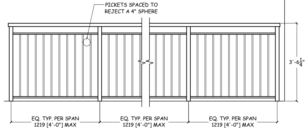
GC201 ELEVATION
