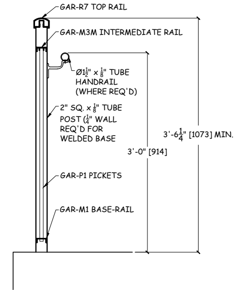
GC201 CROSS SECTION
